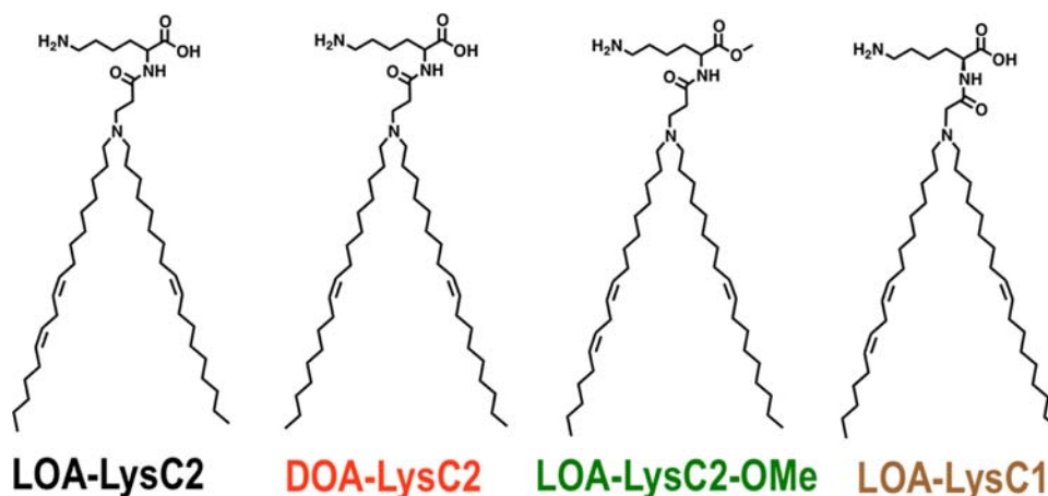
Figure 1. Ionizable lysine-based lipid (ILL) structures.
