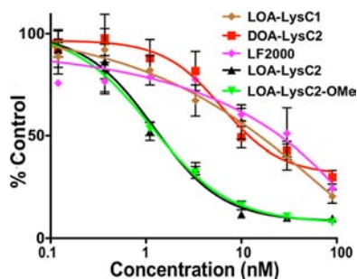
Figure 5. siRNA mediated knockdown of Renilla luciferase in stably transfected HeLa-Luc cells. ILL lipoplexes (40:40:20 ILL/Chol/DOPE) at N/P = 10 were used for all experiments.
