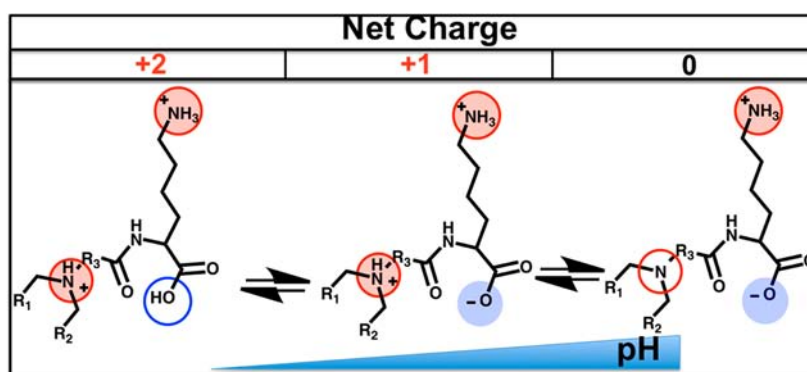
Figure 2. Theoretical pH-dependent ionization of ILL.
