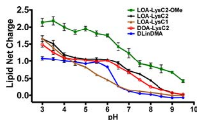
Figure 3. pH-dependent ionization of ILL liposomes (40:40:15:5 ILL/Chol/POPC/PEG-DMG).
